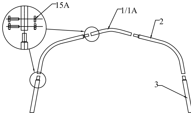
Figure 4 The arch installation
