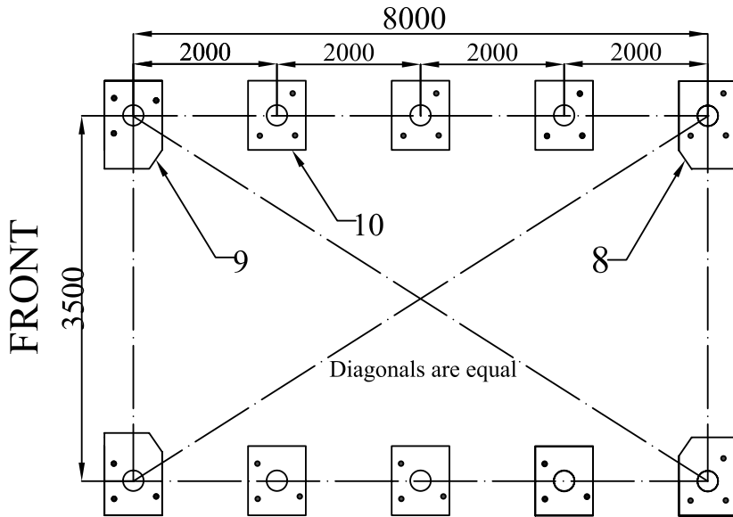
Figure 2 Position of Base Flanges
